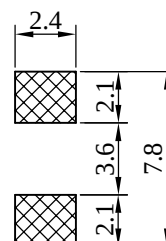
( PCB Pattern )
